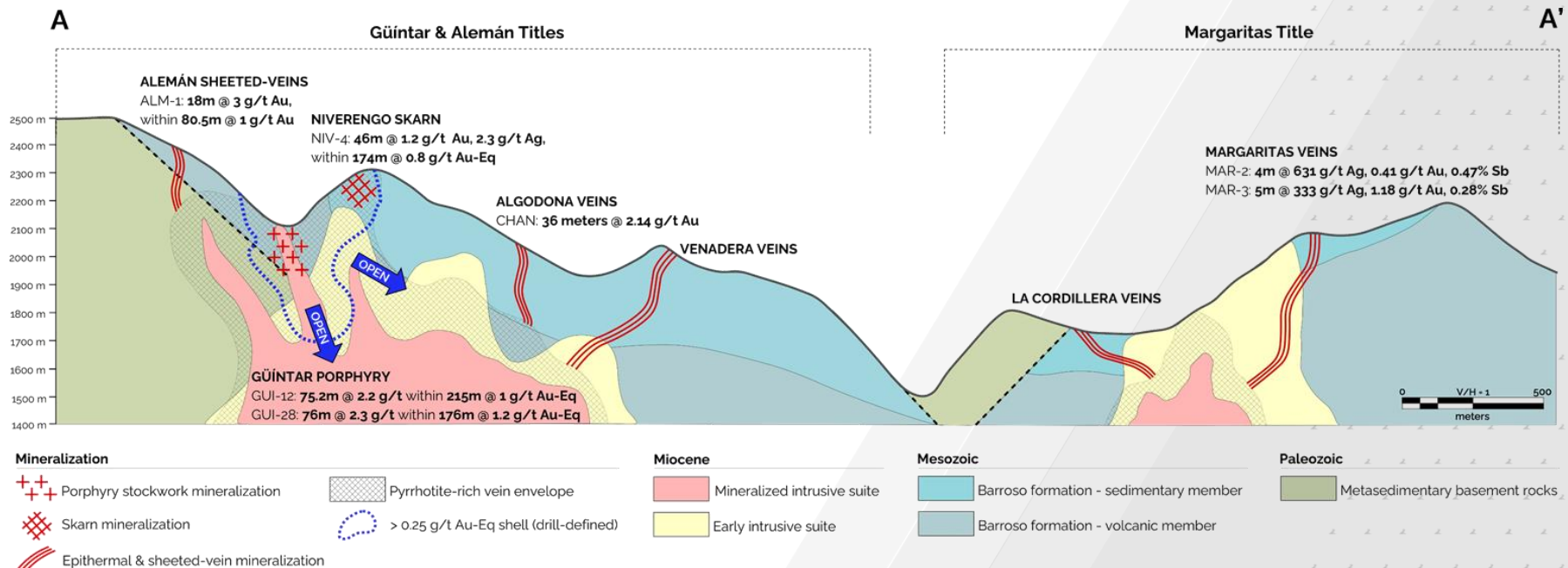
Conceptual geological section A-A' illustrating the interpreted relationship between mineralization styles
